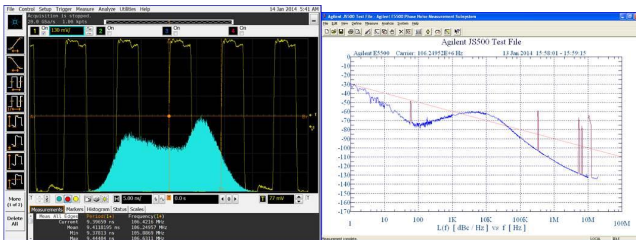
Figure 1. Example Sub-optimal PLL-based XO Phase Noise and Period Jitter
